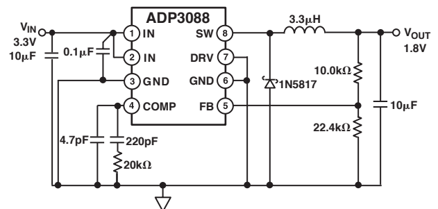
Figure 1. Typical Application
